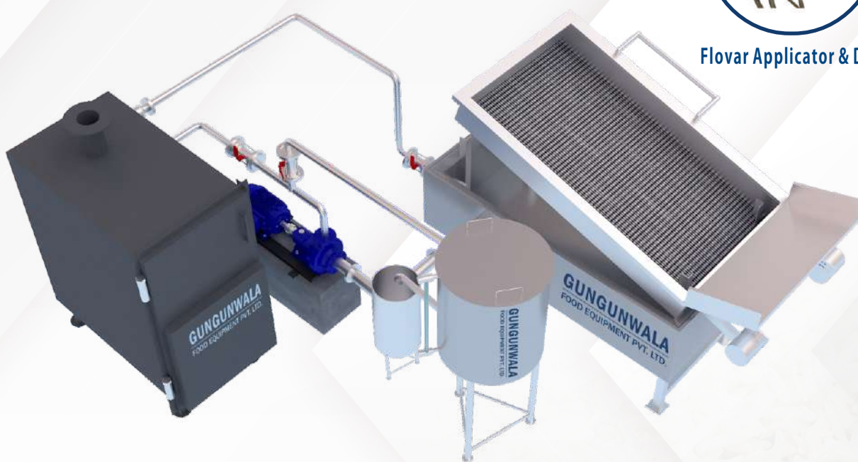
Rectangular Fryer With External Heat Exchanger Diesel/ Gas / Pellets Burner
